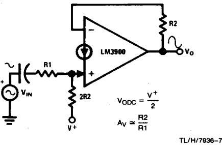
Non-Inverting Amplifier
