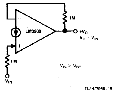
Buffer Amplifier
