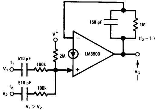
Low-Frequency Mixer
