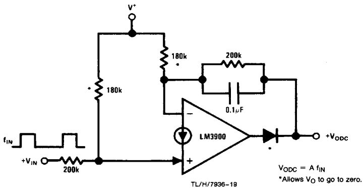
Tachometer
