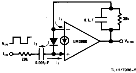
Frequency-Doubling Tachometer
