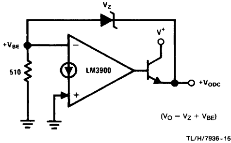
Voltage Regulator
