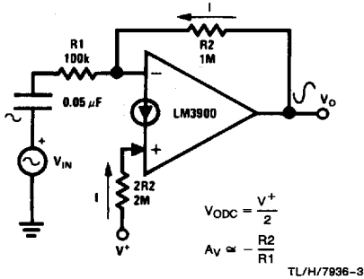
Inverting Amplifier
