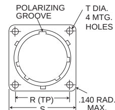
RECEPTACLE ASSEMBLY
