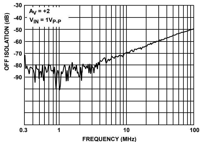
FIGURE 20. OFF ISOLATION
