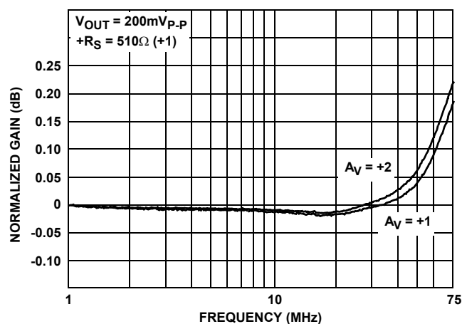
FIGURE 19. GAIN FLATNESS
