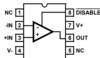
HFA1145 (SOIC) TOP VIEW
