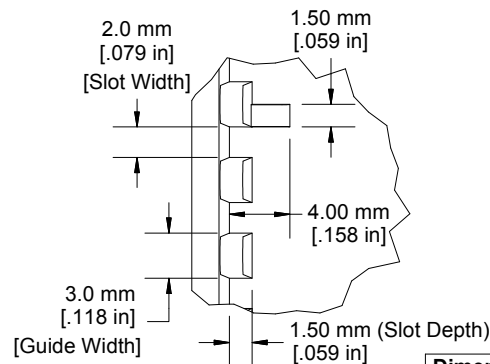
Top View - Interior Features
