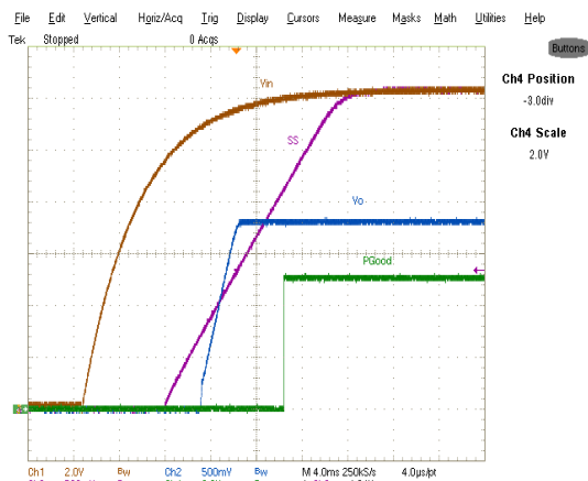
Fig. 18. Start up at 2A Load, Ch_1: V_{in} , Ch_2: V_o , Ch_3: V_{ss} , Ch_4: P_{Good}
