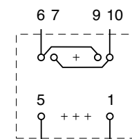
Recommended layout for transformers with 1 secondary winding
