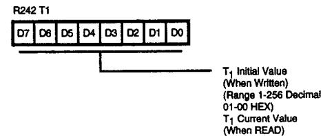
Figure 38. Counter Timer 1 Register (F2 H : Read/Write)
