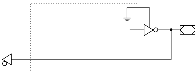
Dedicated Input Configuration for Simple Mode
