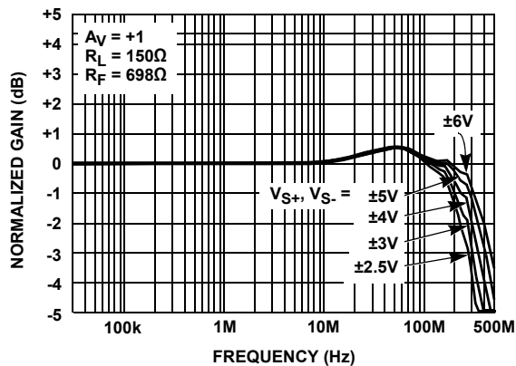
FIGURE 6. FREQUENCY RESPONSE FOR VARIOUS \pm V_S
