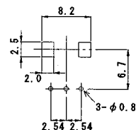
PCB Pattern
