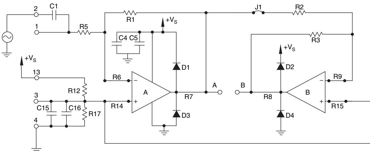
Figure 5 Single Supply Bridge
