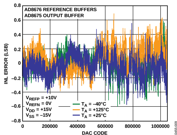
Figure 8. Integral Nonlinearity Error vs. DAC Code, \pm 10 V Span, \times 2 Gain Mode
