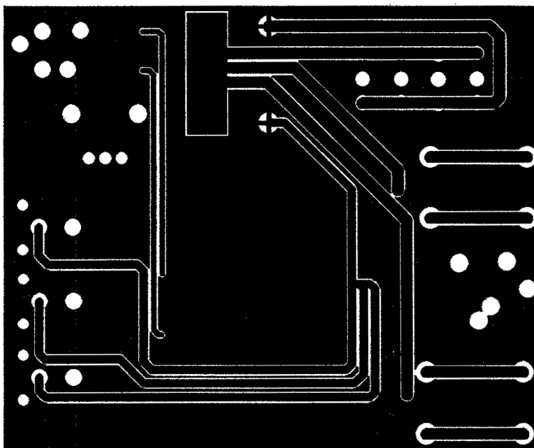
Figure 57. Bottom Layer LQ
