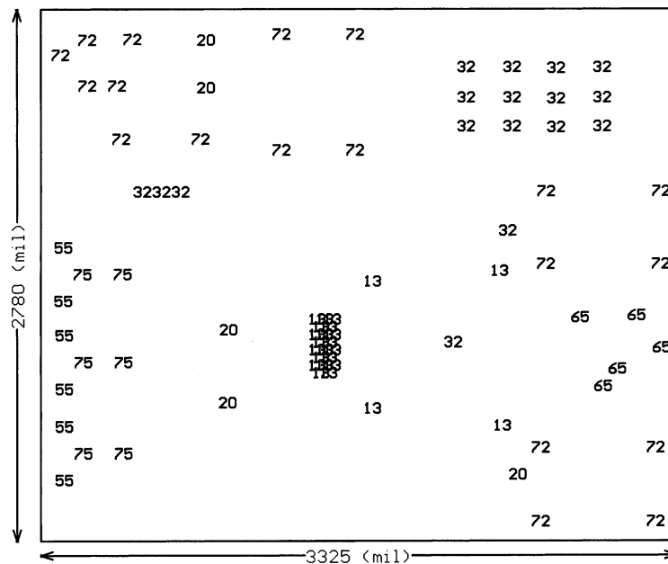
Figure 61. Drill Drawing
