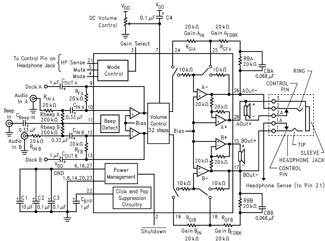
Figure 4. Typical Application Circuit ( MT / MH Package Pinout )
