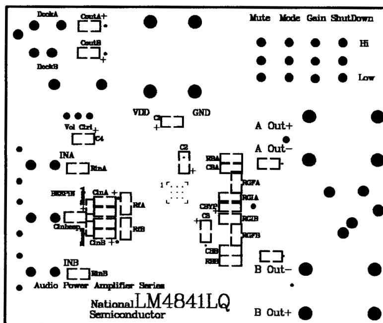
Figure 55. Top Layer SilkScreen
