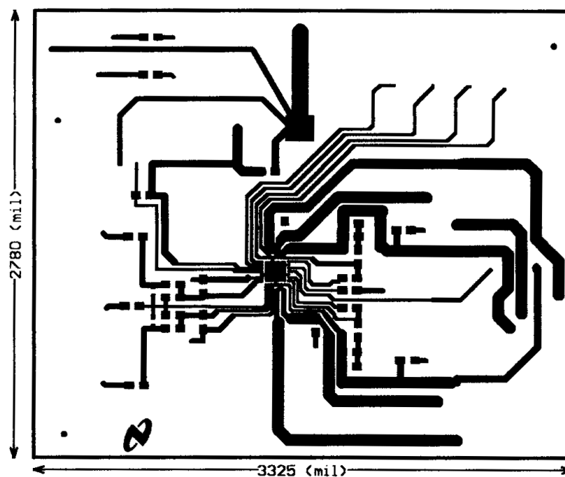
Figure 56. Top Layer LQ
