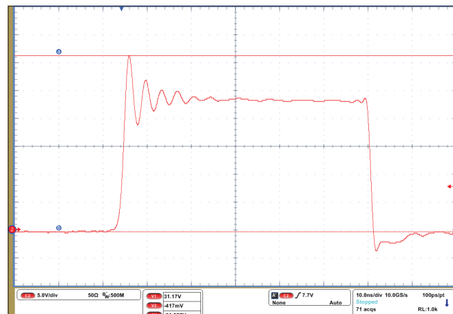
Figure 4: Typical Switch node voltage for a 24 V to 1.2 V/20 A (1 MHz) Buck converter
