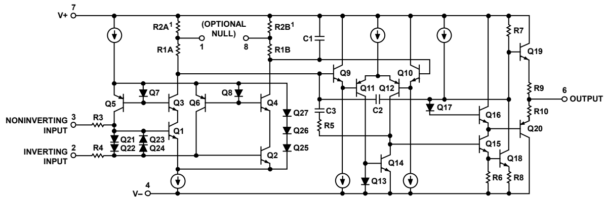
Figure 39. Simplified Schematic
