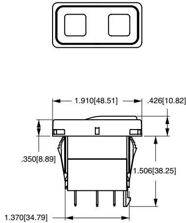
10 TERMINAL BASE W/O BARRIERS
