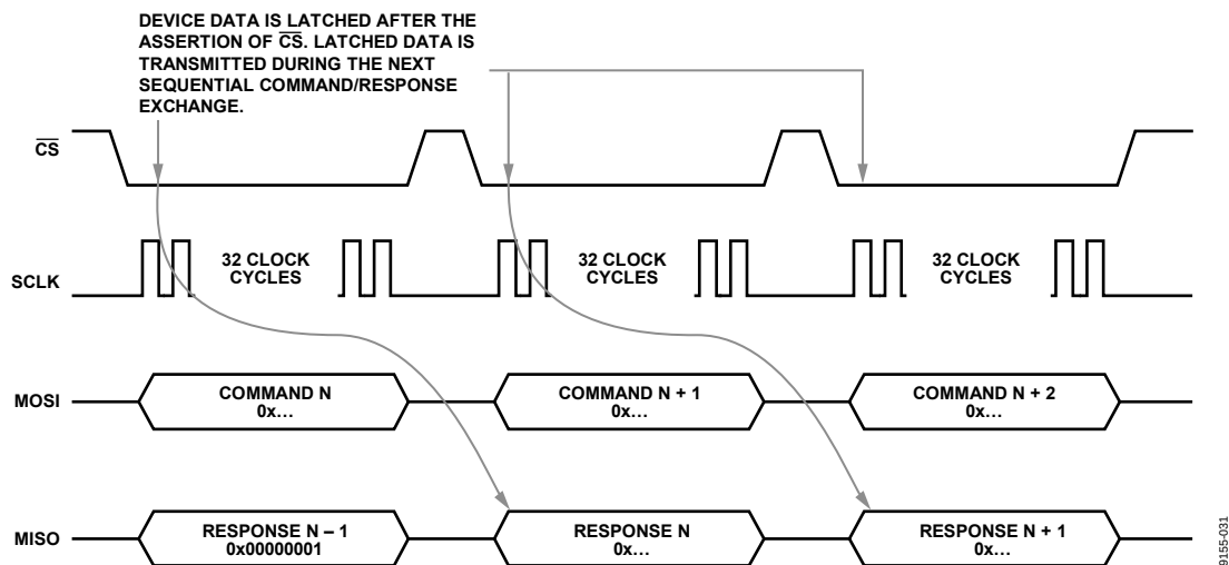
Figure 29. Device Data Latching
