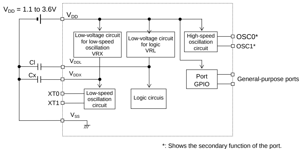
Figure 26-1 Configuration of Power Supply Circuit
