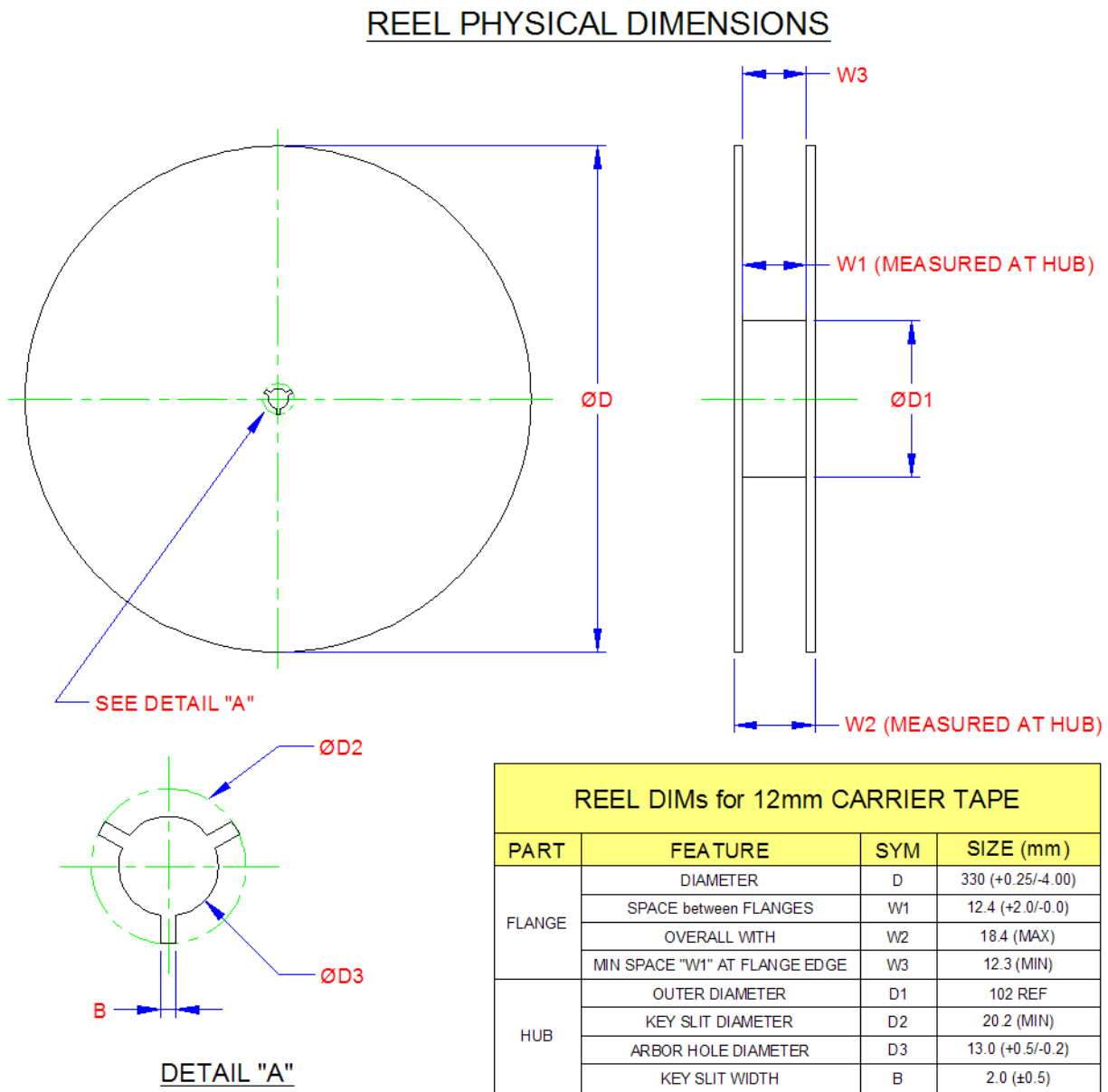
Figure 8.2 Reel Dimensions for 12mm Carrier Tape
