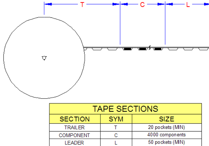
Figure 8.3 Tape Length and Part Quantity
