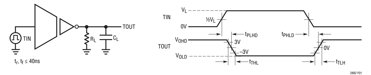
Figure 1. Driver Slew Rate and Timing Measurement
