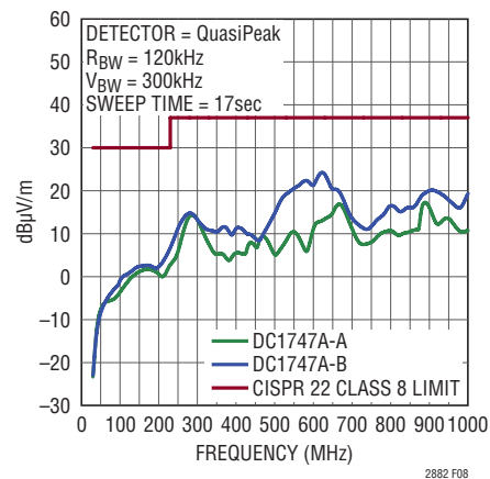
Figure 8. Low EMI Demo Board Emissions
