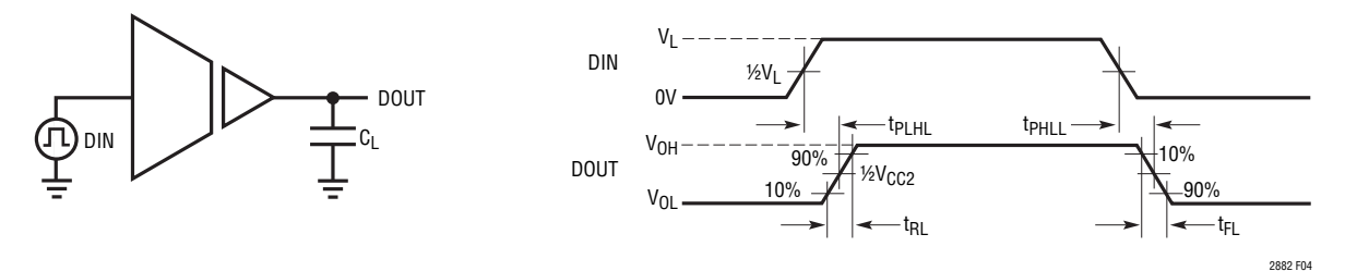
Figure 4. Auxiliary Channel Timing Measurement
