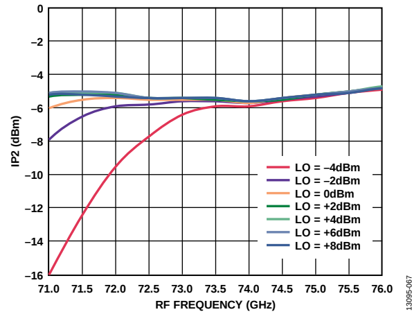
Figure 66. Input IP2 vs. RF Frequency at Various LO Powers, I_{FIN} = 5 dBm, IF = 1000 MHz, USB
