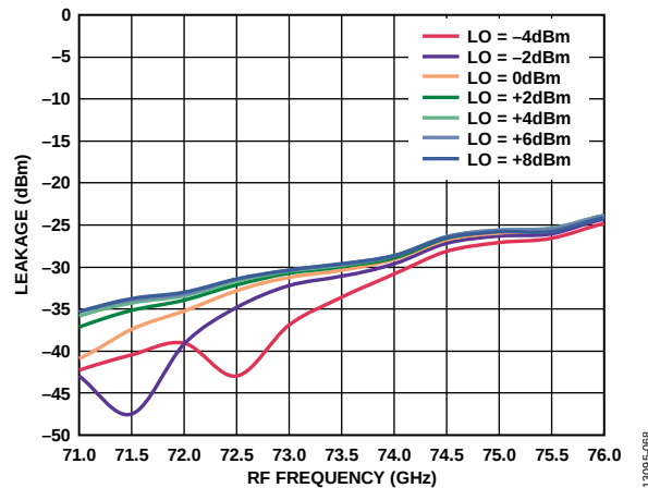
Figure 67. 6x LO Leakage at RFOUT vs. RF Frequency at Various LO Powers, I_{FIN} = 5 dBm, IF = 1000 MHz, USB
