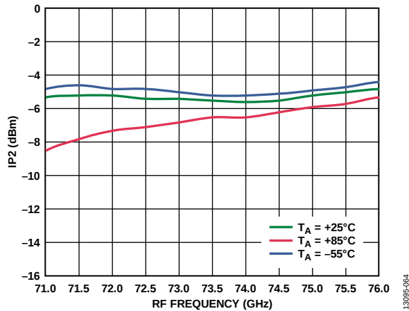
Figure 63. Input IP2 vs. RF Frequency at Various Temperatures, I_{FIN} = 5 dBm, LO = 2 dBm, IF = 1000 MHz, USB
