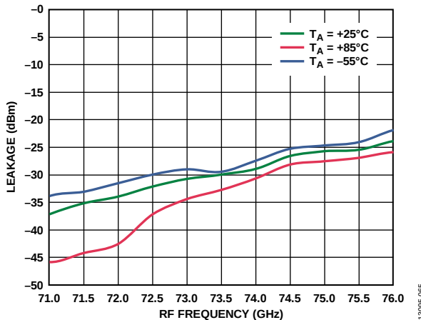
Figure 64. 6x LO Leakage at RFOUT vs. RF Frequency at Various Temperatures, I_{FIN} = 5 dBm, LO = 2 dBm, IF = 1000 MHz, USB
