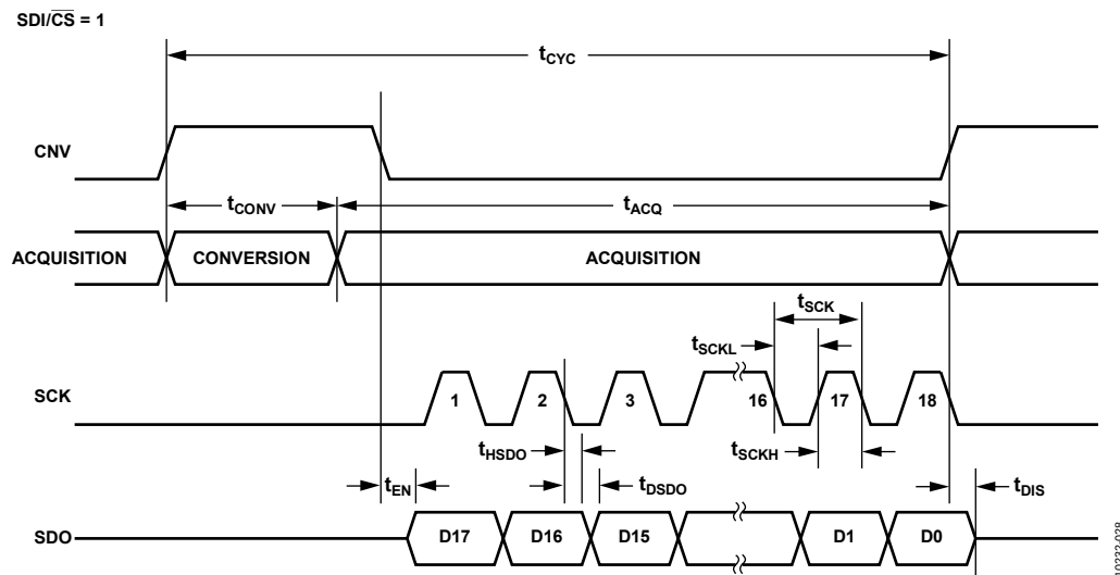
Figure 32. \overline{\text{CS}} Mode, 3-Wire Serial Interface Timing ( \text{SDI} High)
