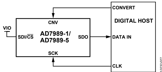
Figure 31. \overline{\text{CS}} Mode, 3-Wire Connection Diagram ( \text{SDI} High)
