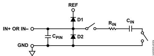
Figure 27. Equivalent Analog Input Circuit
