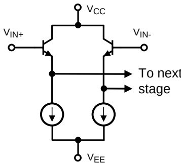
Figure 3. Input Stage
