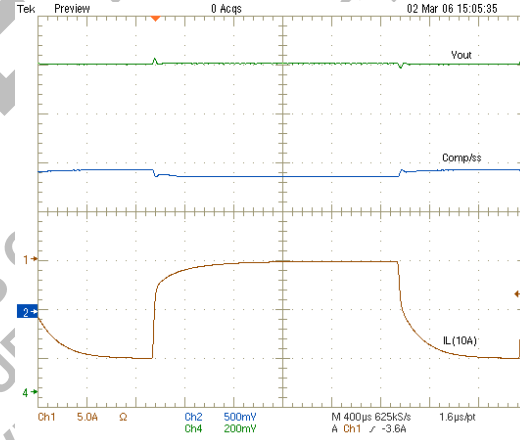
Figure 19. Transient Response
