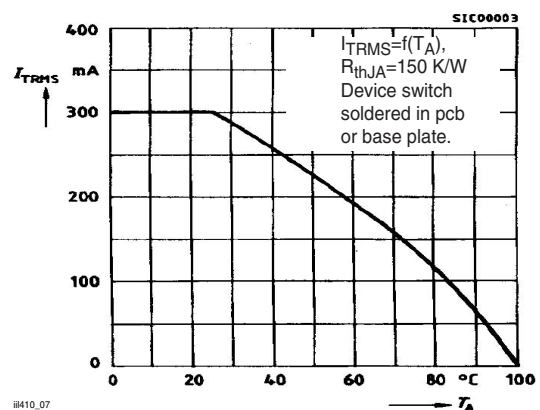
Figure 7. Current Reduction
