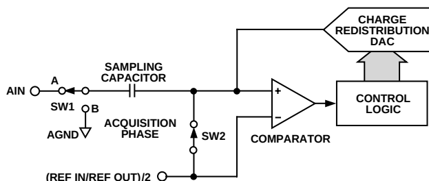
Figure 5. ADC Acquisition Phase
