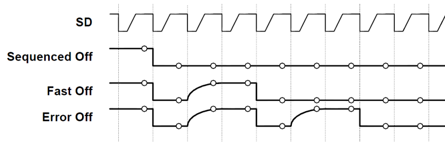
Figure 39. OK Severity Encoding Waveforms
