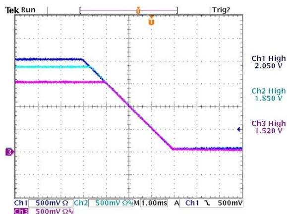
Figure 25. Tracking Turn-Off. Falling Slew Rate is 0.5V/ms.
