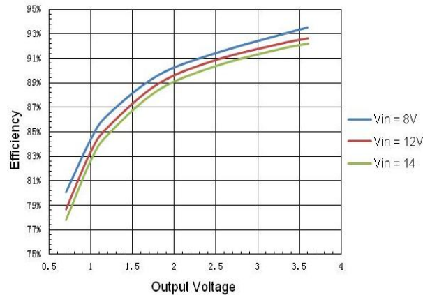
Figure 7: Efficiency vs. Output voltage for converter DP7130, with 30A load, input voltage at 8, 12 and 14V, at T_a = 25^\circ\text{C} .
