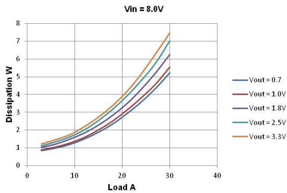
Figure 8: Power dissipation vs. load for converter DP7130, with V_{in} = 8.0\text{V} in T_a = 25^\circ\text{C} .
