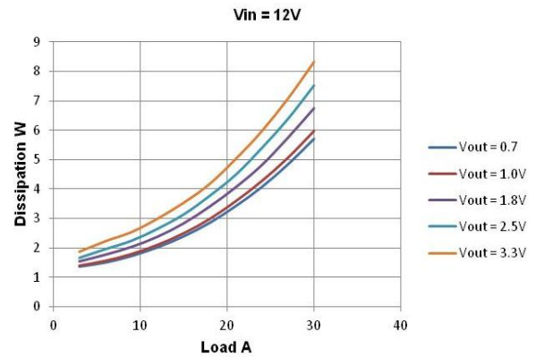
Figure 9: Power dissipation vs. load for converter DP7130, with V_{in} = 12\text{V} T_a = 25^\circ\text{C} .
