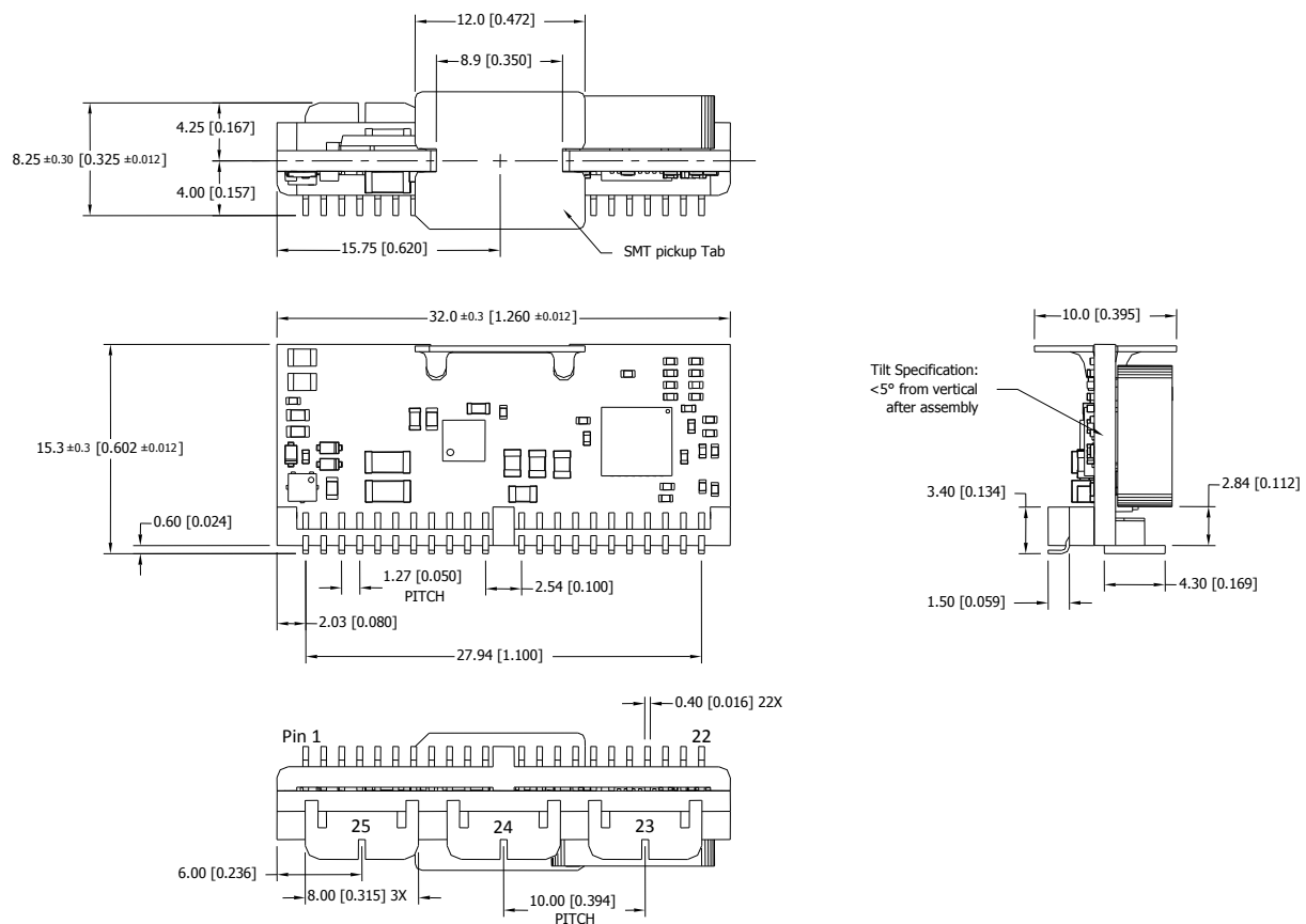
Figure 55: Mechanical Drawing
