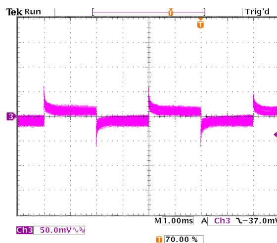
Figure 48. Transient Response with Regulation set to 1.89 mv/A.
