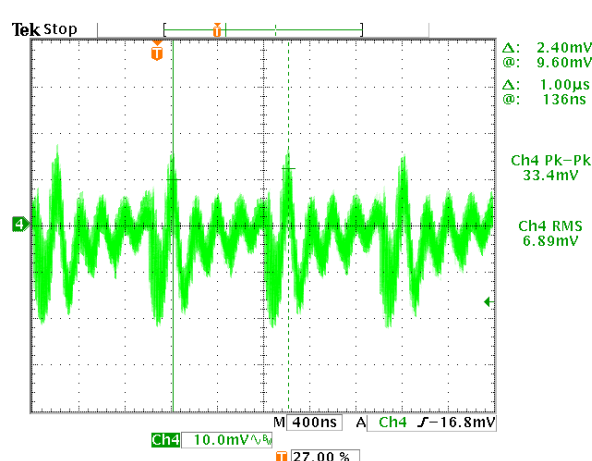
Figure 43. Input Voltage Noise with Interleave
