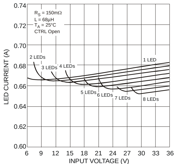
Figure 17 670mA LED Current vs. Input Voltage
