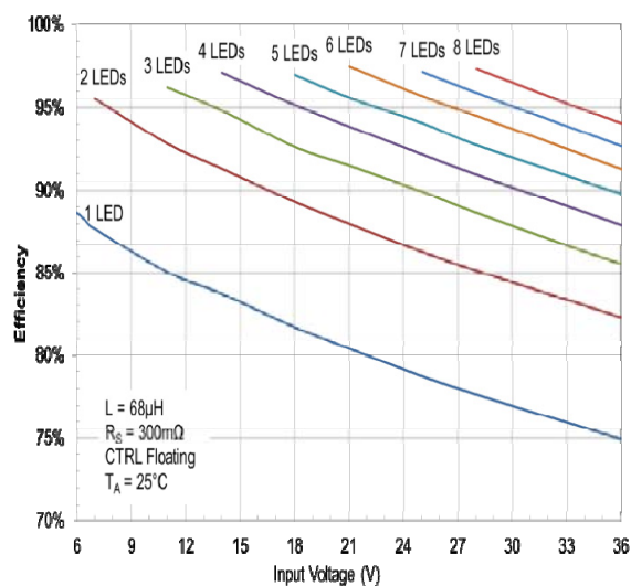
Figure 14 Efficiency vs. Input Voltage
