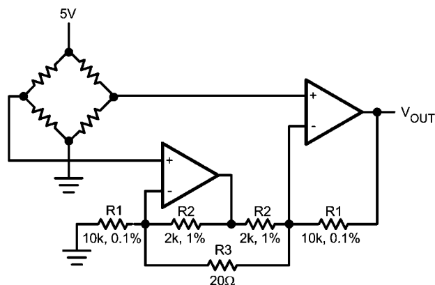
FIGURE 4. Precision Strain Gauge Amplifier
