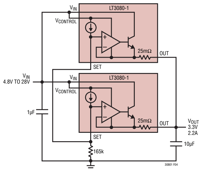
Figure 4. Parallel Devices
