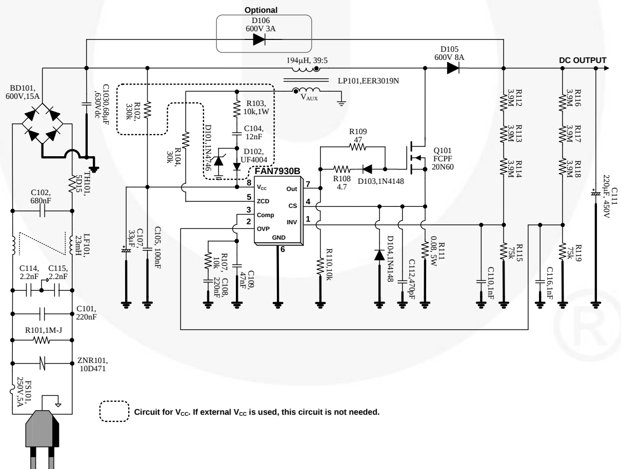
Figure 44. Demonstration Circuit
