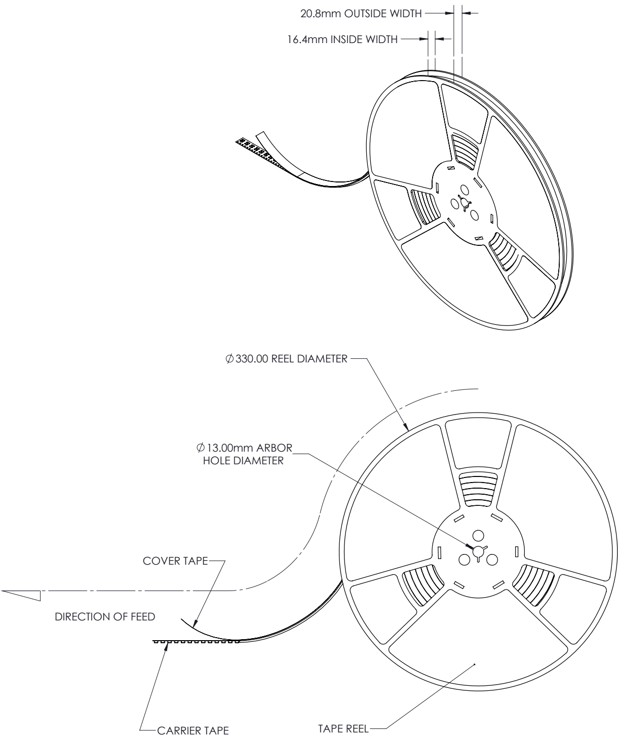
Figure 15. Emitter reel packaging.
