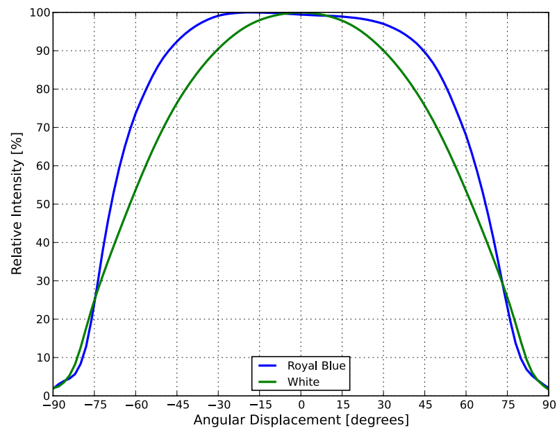
Figure 12. Typical representative spatial radiation pattern.
