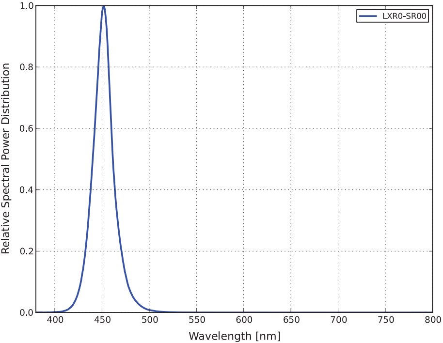
Figure 8. Color spectrum of LXR0-SR00 emitter, integrated measurement.
