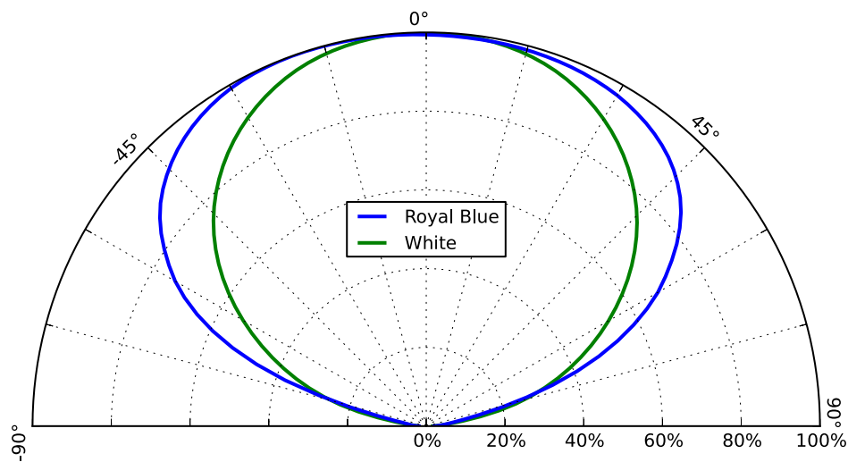
Figure 13. Typical polar radiation pattern.
