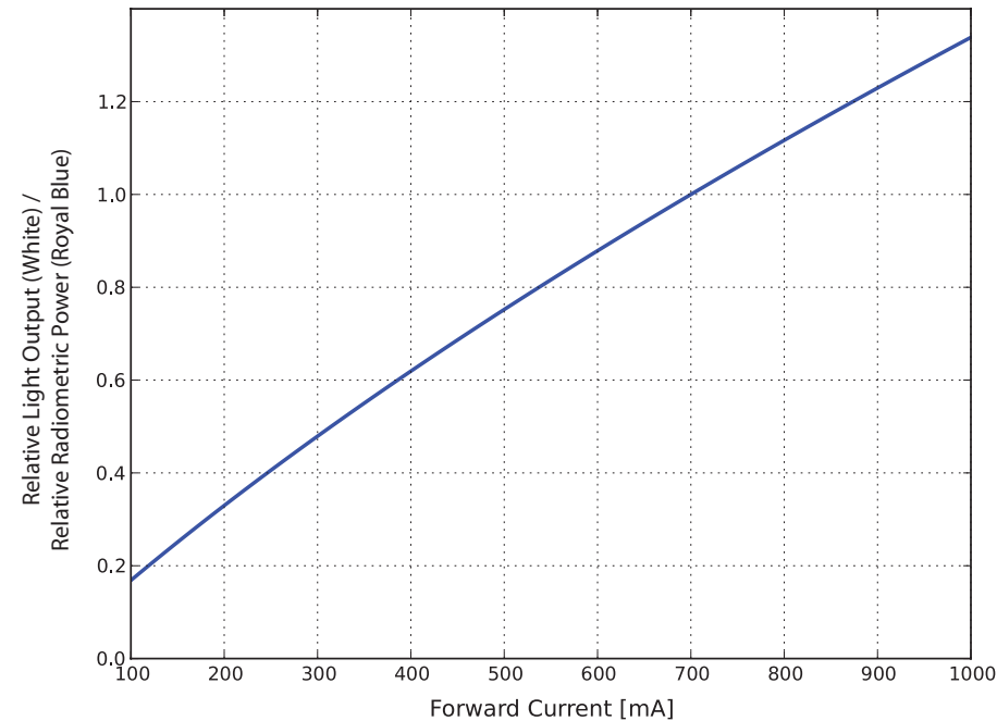
Figure 10. Relative light output vs. forward current.
