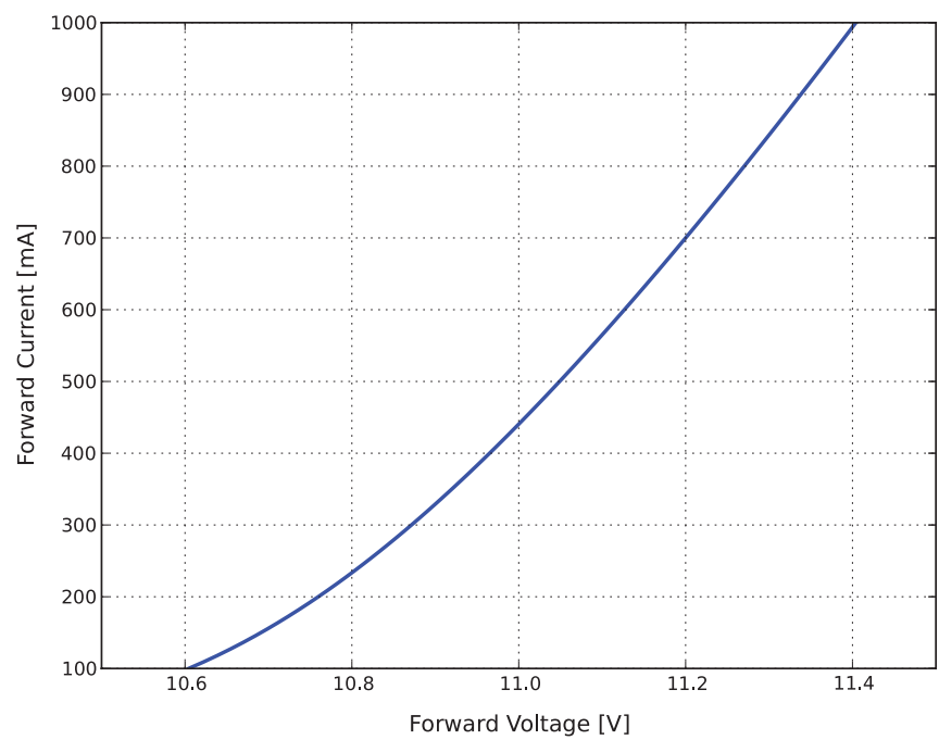
Figure 11. Forward current vs. forward voltage.
