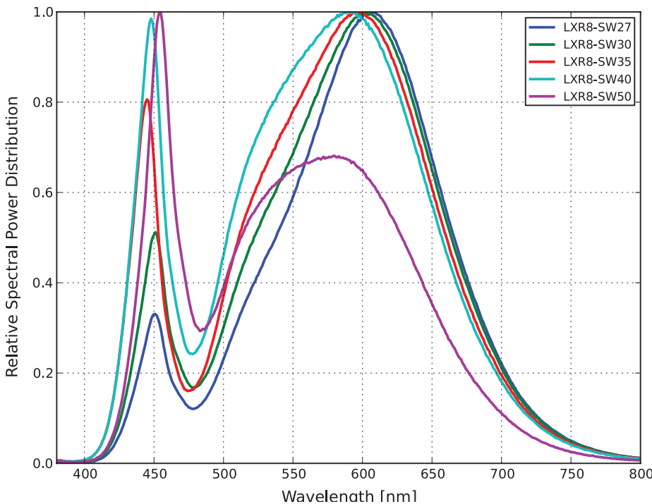
Figure 6. Color spectrum of LXR8-SWxx emitter, integrated measurement.
