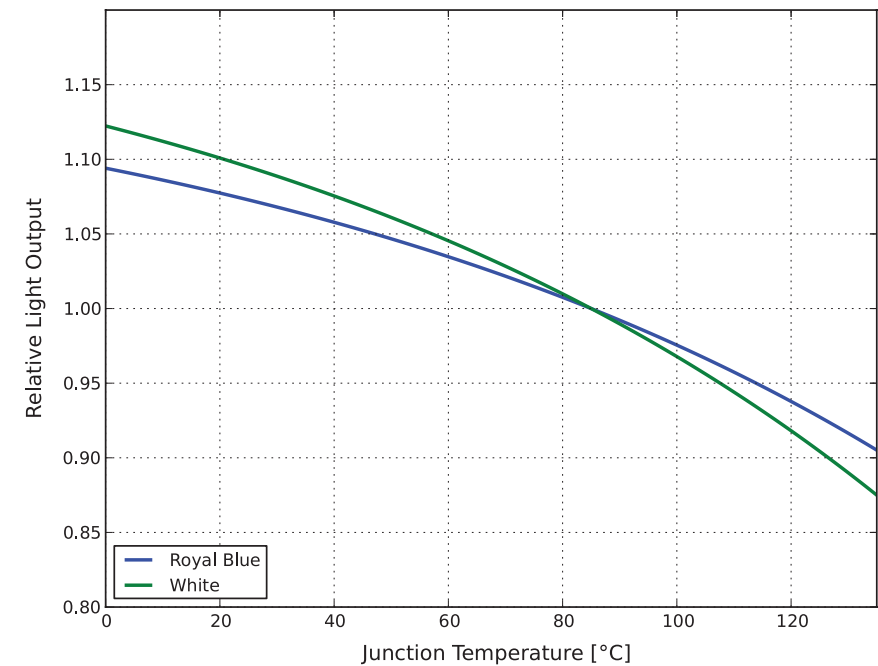
Figure 9. Relative light output vs. junction temperature.
