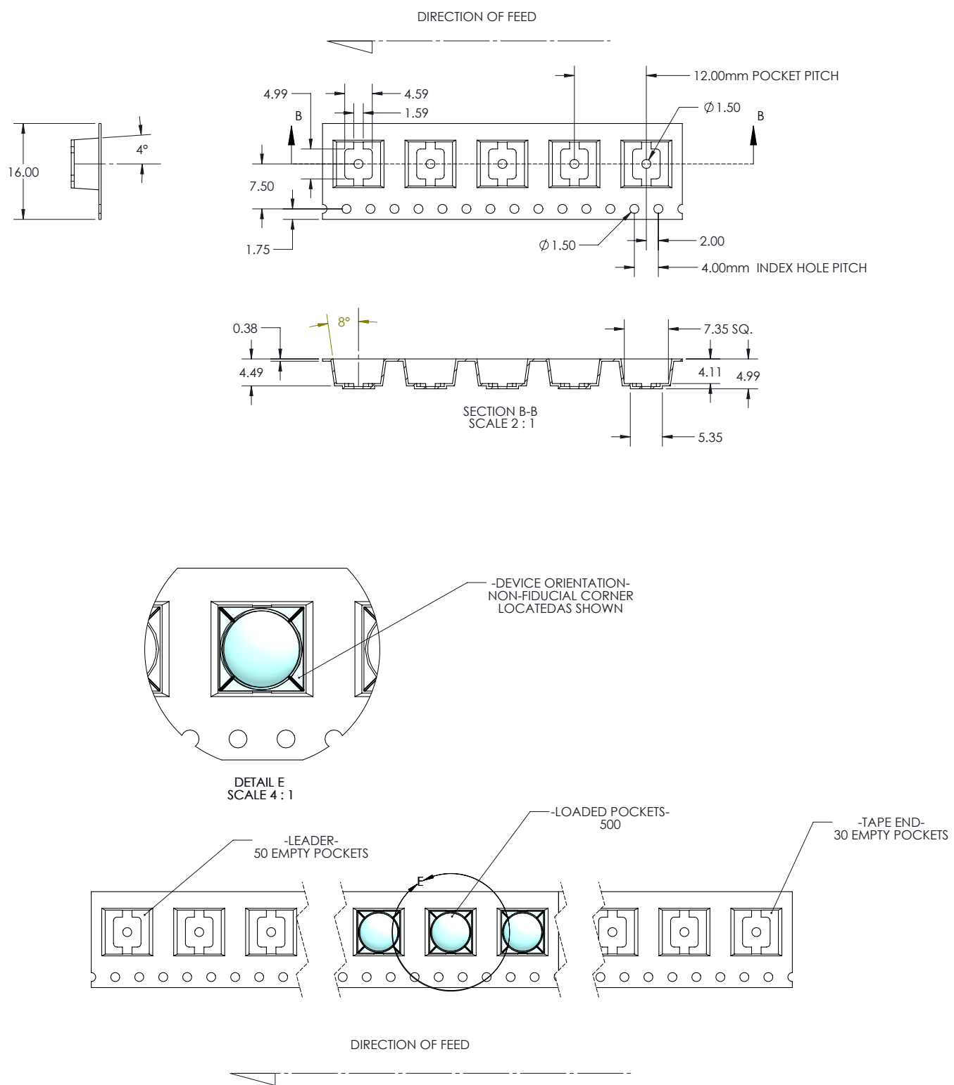
Figure I4. Emitter pocket tape packaging.
