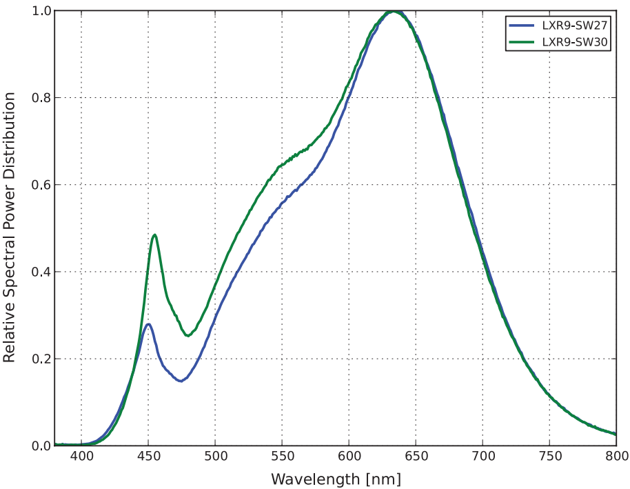
Figure 7. Color spectrum of LXR9-SWxx emitter, integrated measurement.
