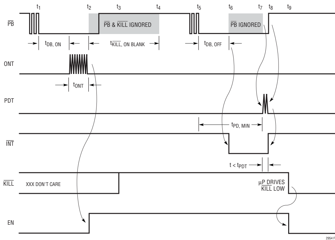
Figure 1. Simplified Power On/Off Sequence for LTC2954-1. \mu P Asserts \overline{\text{KILL}} after an Interrupt
