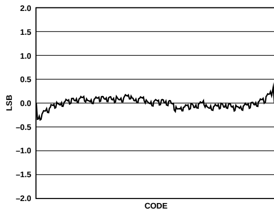
Figure 16. Integral Nonlinearity
