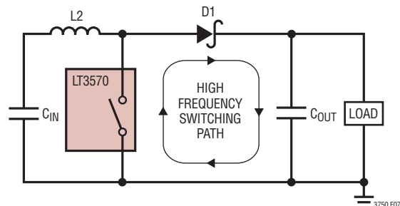
Figure 7. Boost High Speed Switching Path
