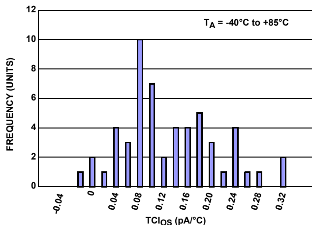
FIGURE 34. TCI_{OS} HISTOGRAM
