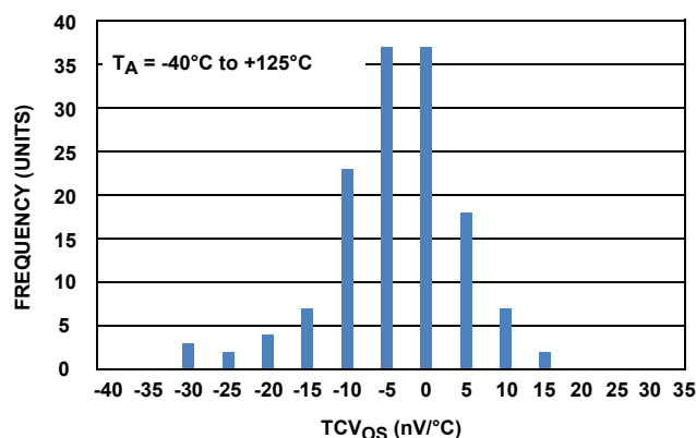
FIGURE 36. TCV_{OS} HISTOGRAM
