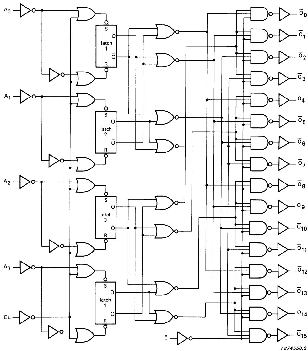
Fig.3 Logic diagram.
