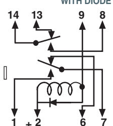
DPDT
