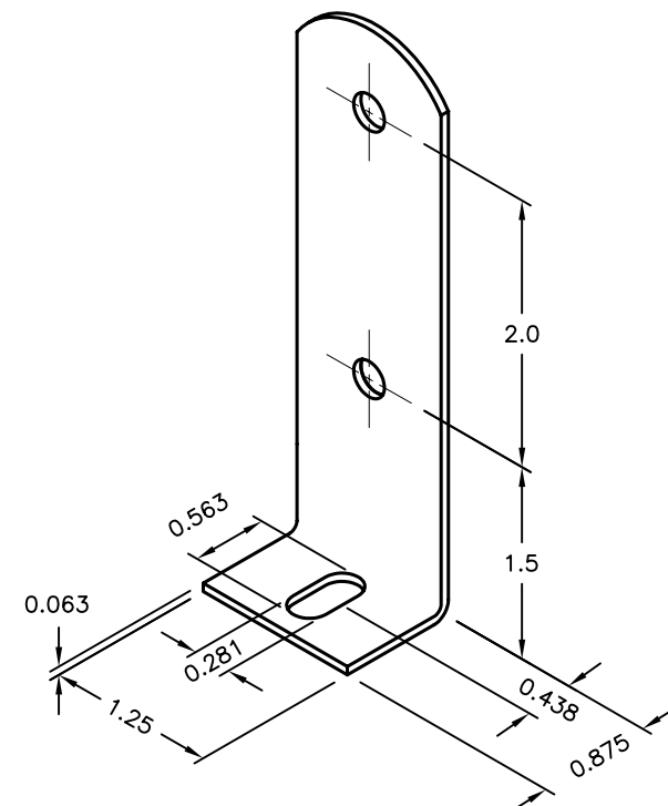
Brackets Dimensions
