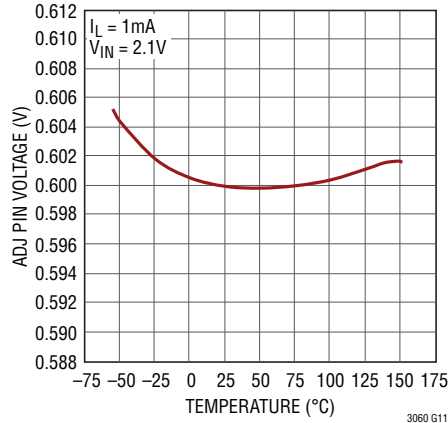
LT3060 ADJ Pin Voltage
