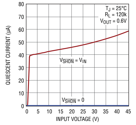
LT3060 Quiescent Current
