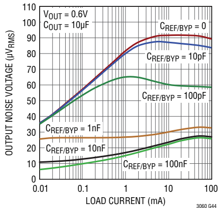
RMS Output Noise vs Load Current vs C_{REF/BYP} , C_{FF} = 0
