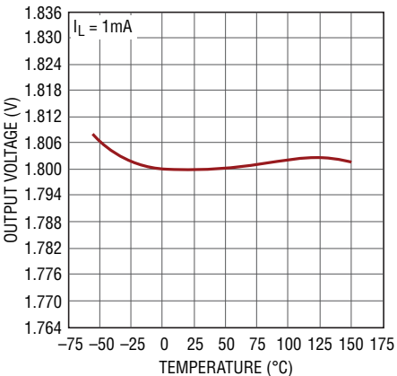
LT3060-1.8 Output Voltage
