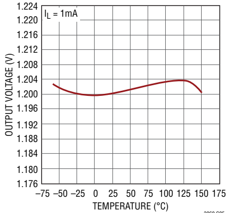
LT3060-1.2 Output Voltage
