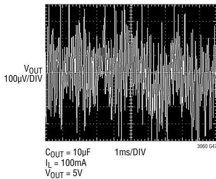
LT3060-5 10Hz to 100kHz Output Noise, C_{REF/BYP} = 10\text{nF} , C_{FF} = 0
