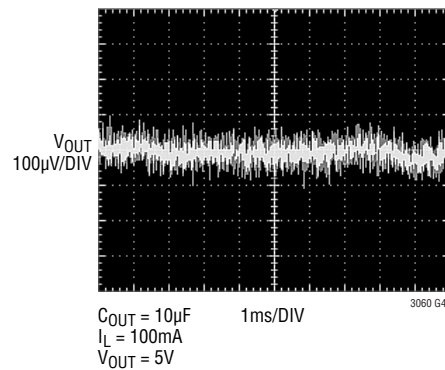
LT3060-5 10Hz to 100kHz Output Noise, C_{REF/BYP} = 10\text{nF} , C_{FF} = 10\text{nF}
