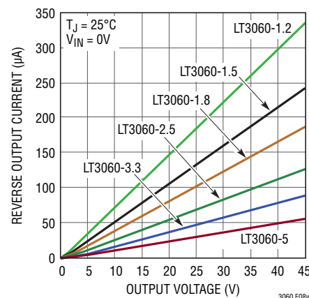
Figure 8. LT3060-1.2/-1.5/-1.8/-2.5/-3.3/-5 Reverse Output Current
