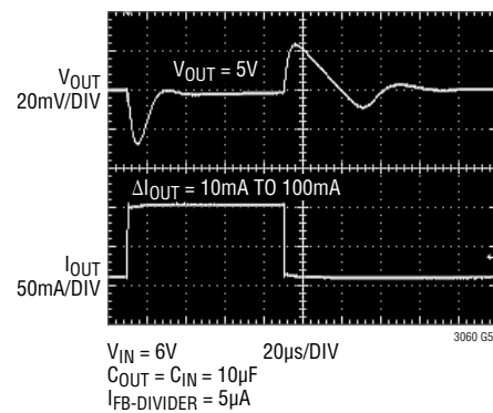
LT3060-5 Transient Response, C_{FF} = 10\text{nF}
