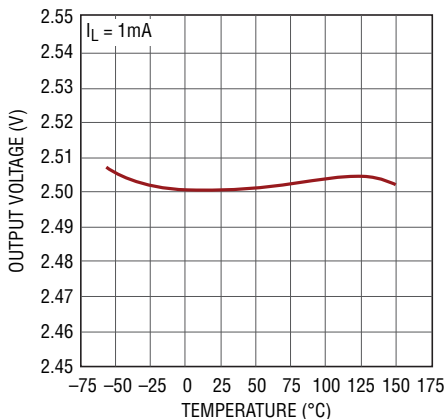
LT3060-2.5 Output Voltage
