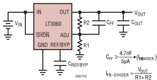
Figure 2. Feedforward Capacitor for Fast Transient Response
