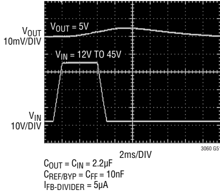
LT3060-5 Transient Response Load Dump
