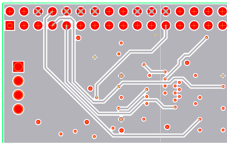
Figure 15– inner layer2 layout
