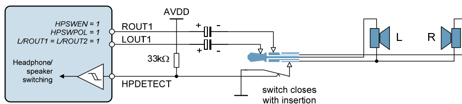
Figure 12 Example Headset Detection Circuit Using Normally-Closed Switch
