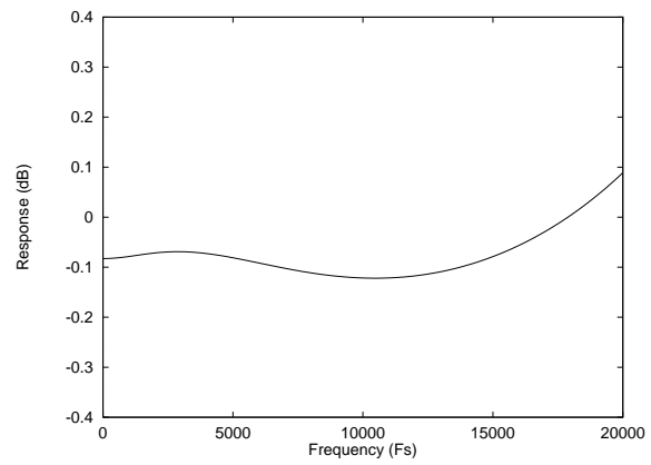
Figure 47 De-emphasis Error (44.1kHz)
