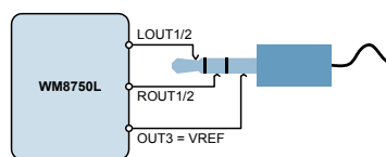
Figure 13 Recommended Headphone Output Configurations
