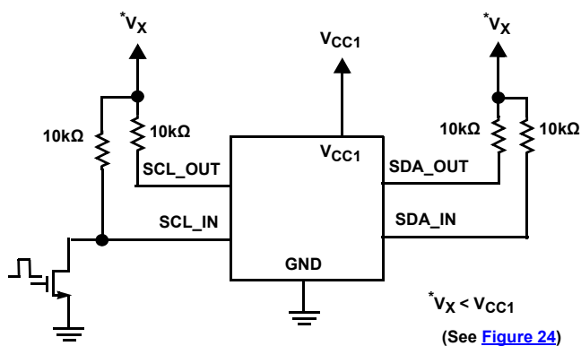
FIGURE 9. ACCELERATOR PULSE WIDTH TEST CIRCUIT
