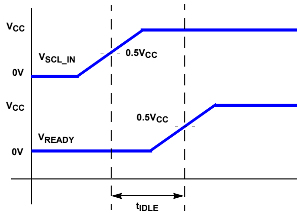
FIGURE 4. BUS IDLE TIME
