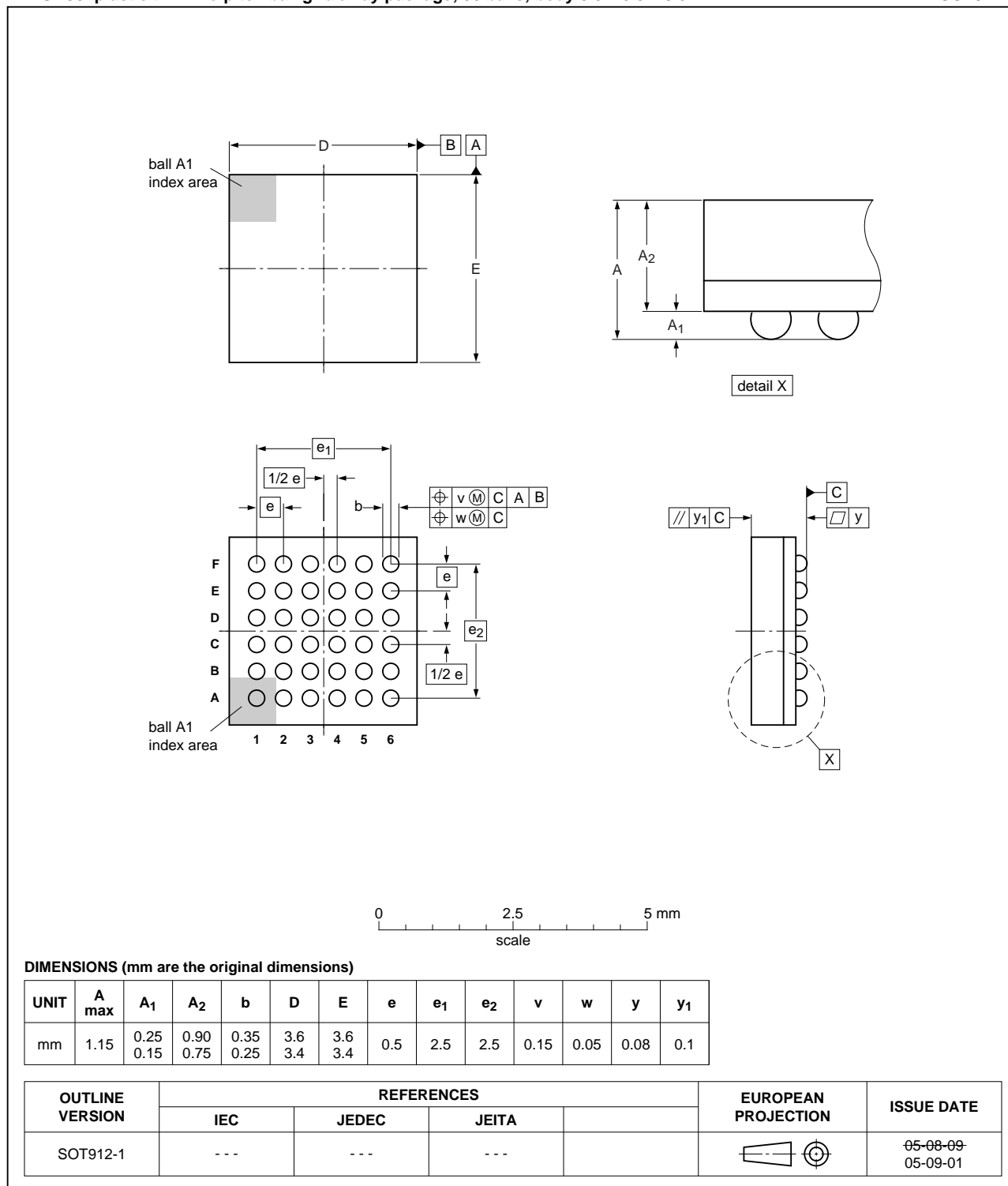
TFBGA36: plastic thin fine-pitch ball grid array package; 36 balls; body 3.5 x 3.5 x 0.8 mm
