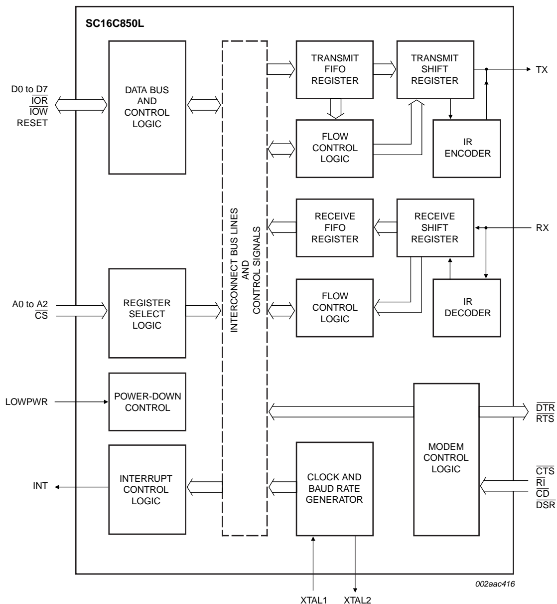
Fig 1. Block diagram of SC16C850L (16 mode)
