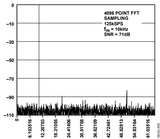
Figure 5. Dynamic Performance
