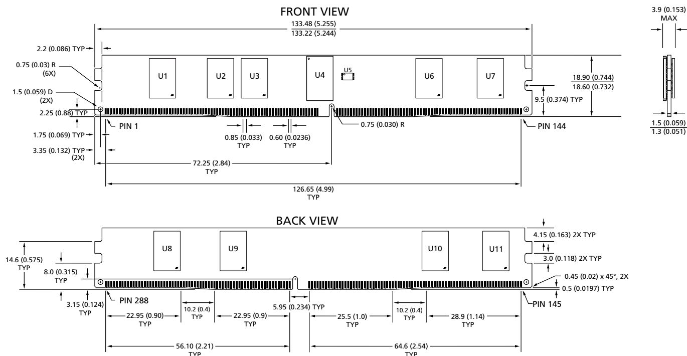
Figure 6: 288-Pin DDR4 RDIMM, PCB 2462
