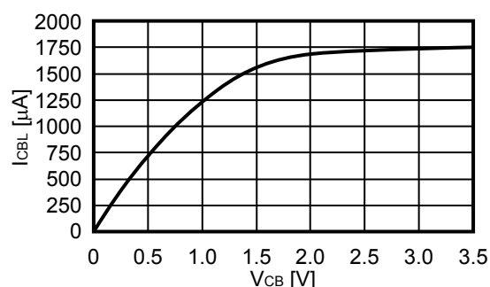
3.4 I_{CBL} vs. V_{CB} ( V_{DS} = 3.5 V)
