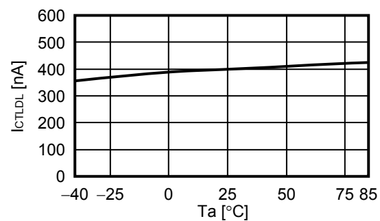
4.2 I_{CTLDL} vs. T_a ( V_{DS} = 3.5 V)
