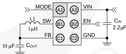
Figure 1. Typical Application
