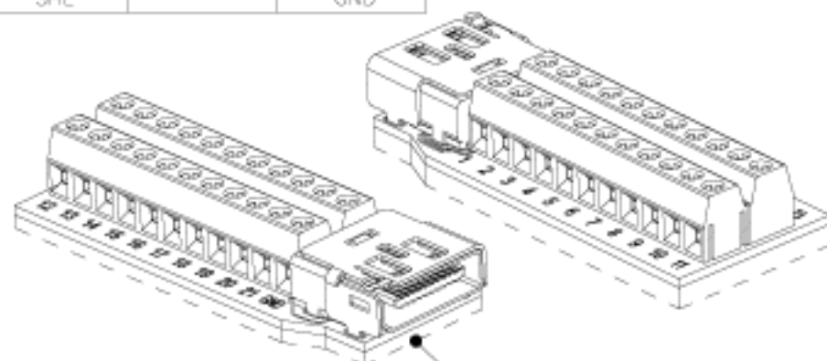
Part name: Adapter DP&HDMI Female to terminal block EVA , T=4mm
