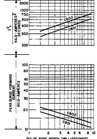
9. SUB-CYCLE SURGE AND I^2t RATING FOLLOWING RATED LOAD CONDITIONS
